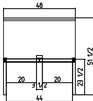
C-U48F-HC TOP VIEW
