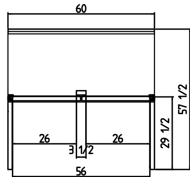
C-U60F-HC TOP VIEW
