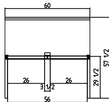
C-U60R-HC TOP VIEW
