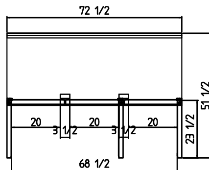
C-U72R-HC TOP VIEW
