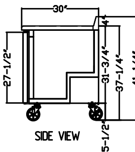
SIDE VIEW (1,2,3) DOORS MODELS
