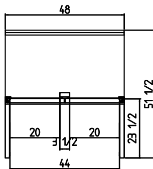
C-U48R-HC TOP VIEW
