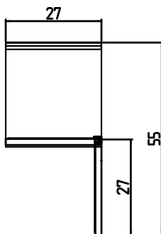
C-U27R-HC TOP VIEW
