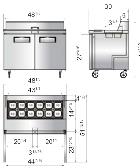
MSF8304GR
