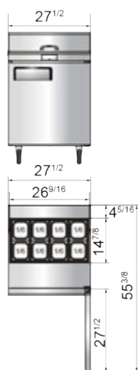
MSF8303GR
