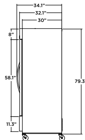
EDJR SIDE EDRF SIDE
