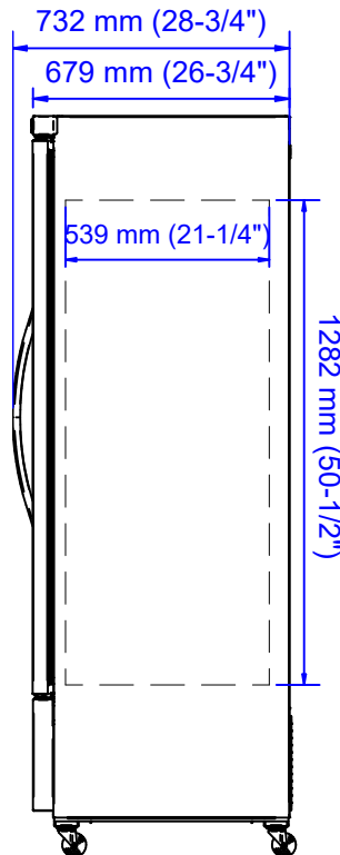
EDJR-17-B-HC SIDE
