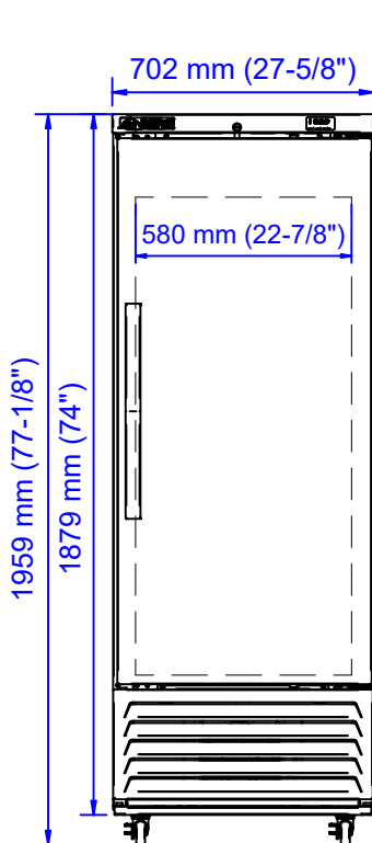
EDJR-17-B-HC FRONT
