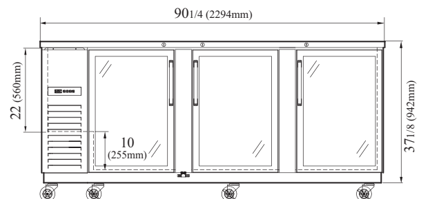
TBB-4SGD-N FRONT VIEW
