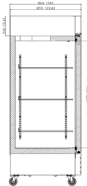
SIDE VIEW FOR BOTH MODELS
